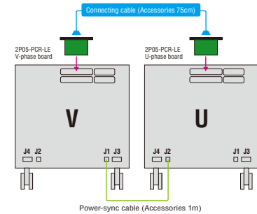
[Example of single phase 3-wire 4 kVA system]
